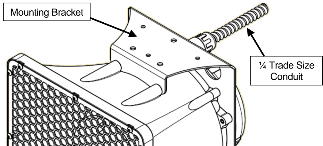
Figure 3: Mounting Bracket
