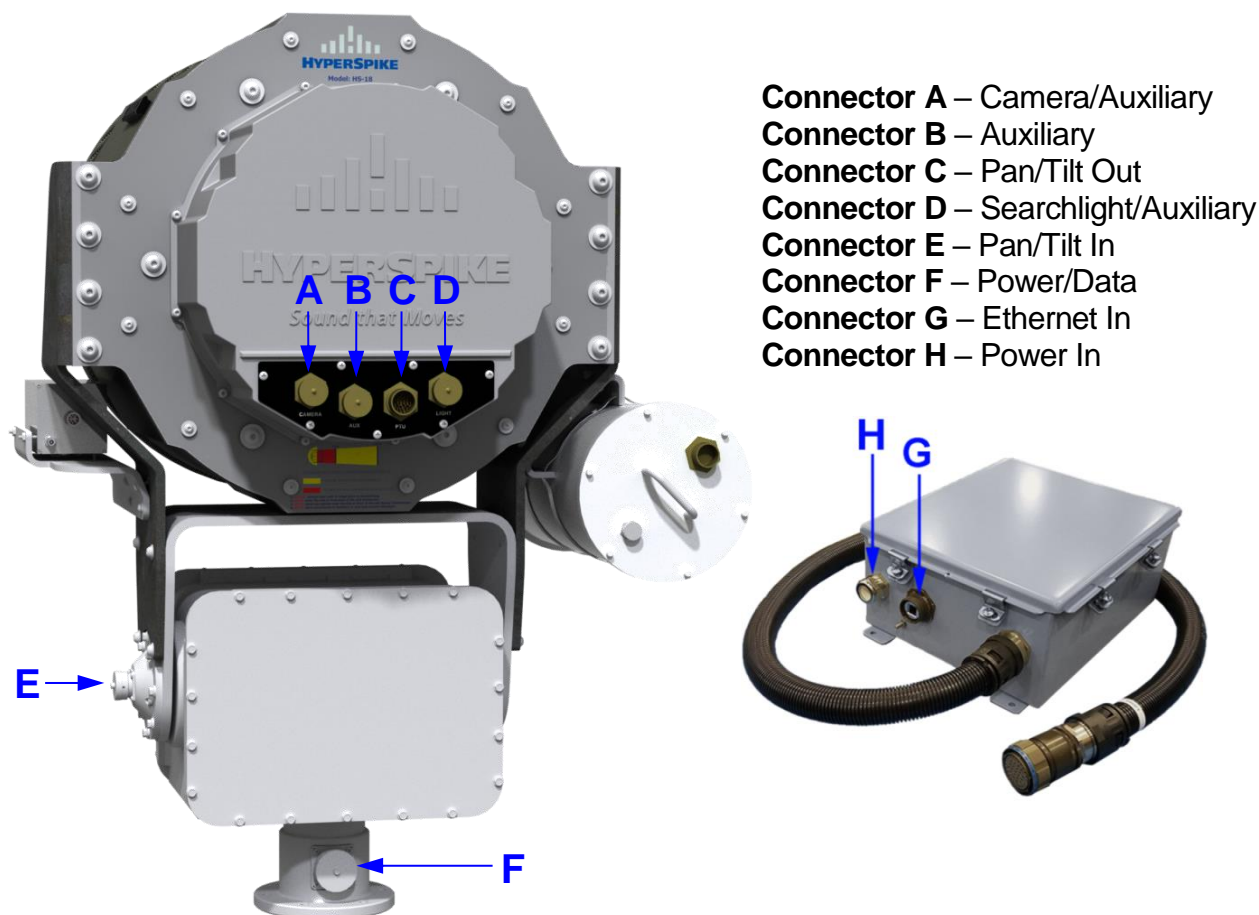
Figure 7: Connector Diagram
