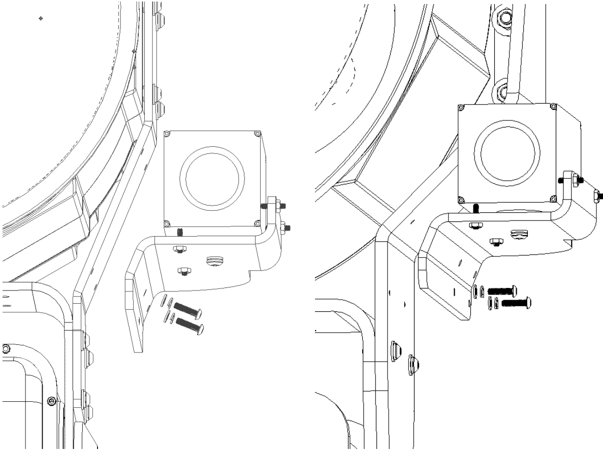
Figure 59: Mounting Camera Bracket to HS-14 RAHD (Left) and HS-18 RAHD (Right)
