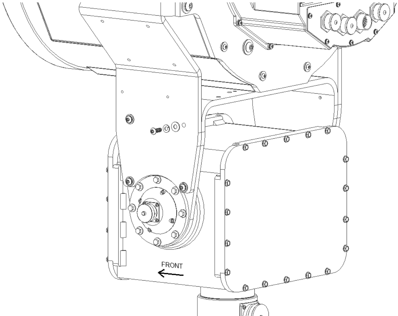
Figure 3: Sound Emitter Head to PTU Assembly
