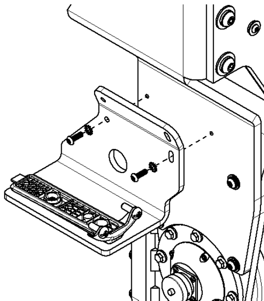
Figure 65: Mounting Camera Bracket to HS-18 RAHD
