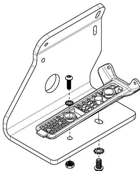
Figure 64: Camera Base to Bracket Installation
