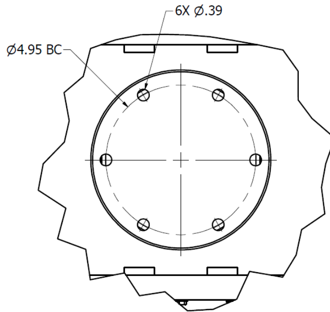
Figure 5: HS-18 RAHD Interface Mounting Dimensions
