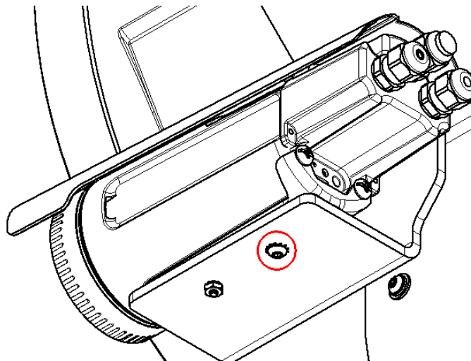
Figure 70: Pan Adjustment
