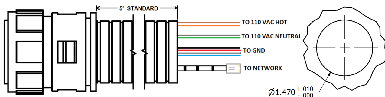
Figure 8: Wiring Diagram for 110 VAC – No Transformer and Hole Size
