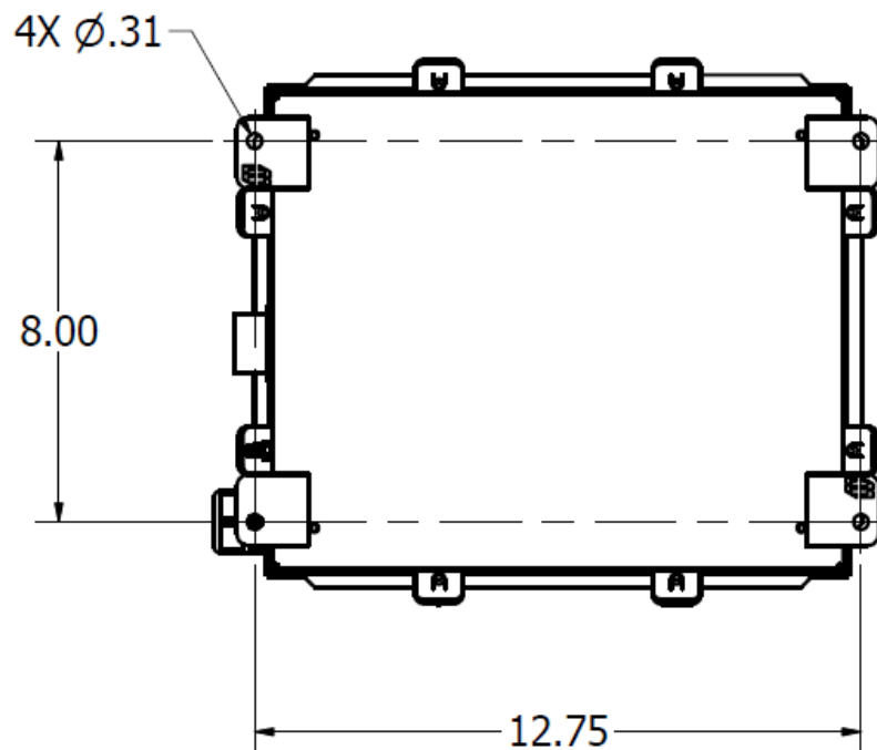
Figure 6: Transformer Box Interface Mounting Dimensions
