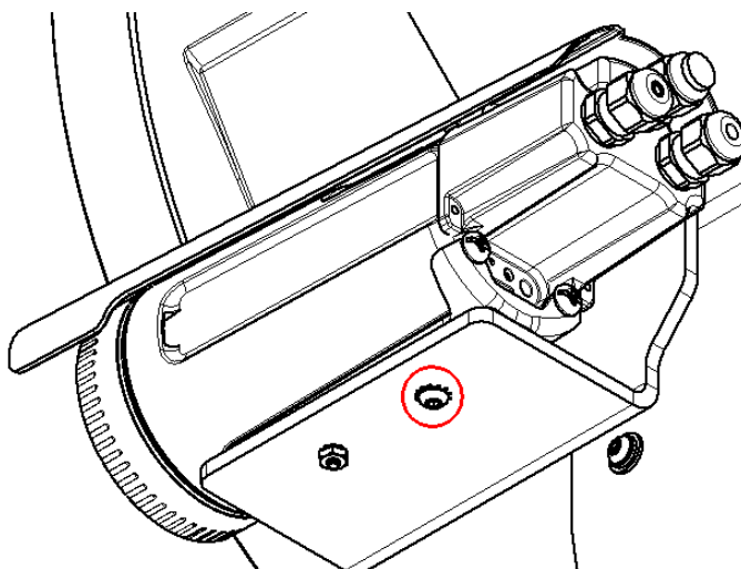
Figure 68: Pan Adjustment
