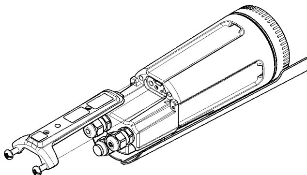
Figure 63: Camera Base Removal
