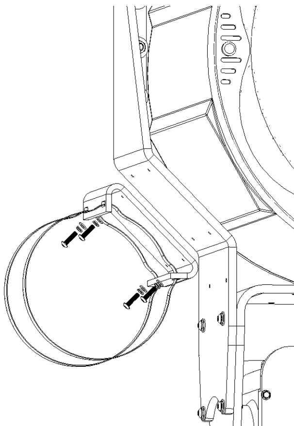
Figure 55: Mounting Light Bracket to HS-18 RAHD
