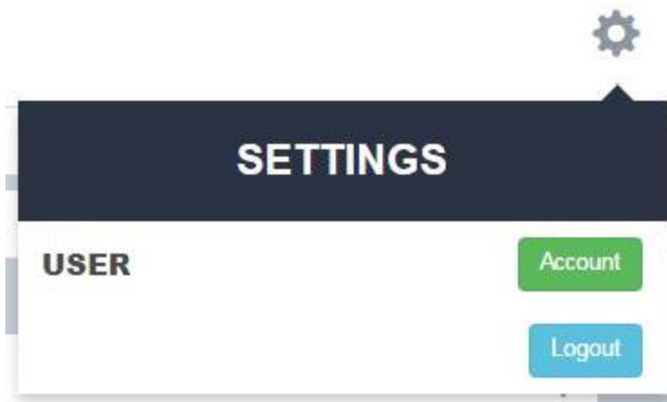
Figure 47: Settings Menu
