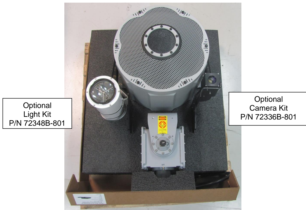
Figure 2: HS-18 RAHD – In Packaging
